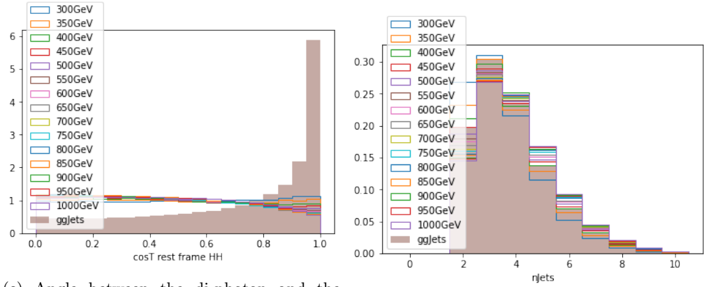
(c) Angle between the di-photon and the beam axis in the di-Higgs rest frame.
