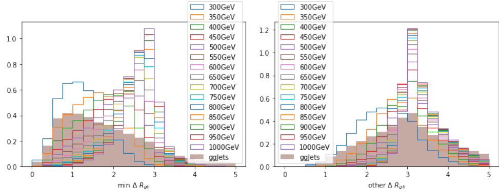
(e) \Delta R between the closest photon-jet pair.
