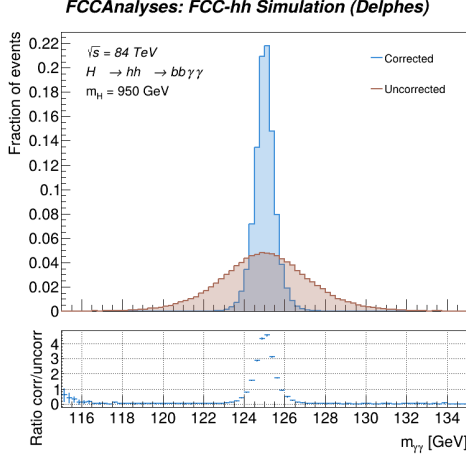
Fig. 3: Impact of the correction to the di-photon invariant mass resolution for an example H \rightarrow hh \rightarrow b\bar{b}\gamma\gamma signal with a mass of 950 GeV.
