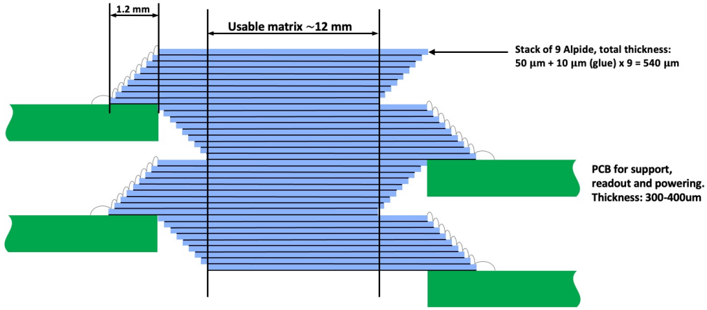
Figure 3.5: Cross-sectional view of Pixel Chamber composed by an assembly of 24 A9 stacks.
