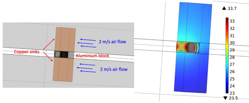
Figure 4.11: Left: Setup for cooling emulation. Right: Stabilized temperature of the mock Pixel Chamber with 2 m/s air flow cooling and cooper heat sink.
