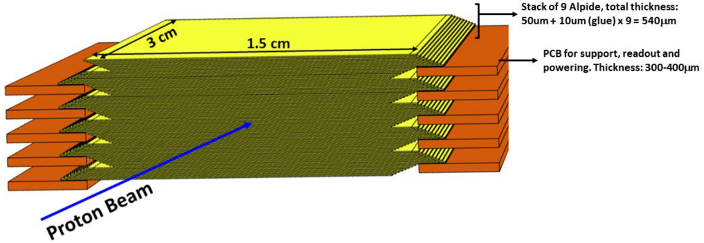
Figure 1.6: Pixel Chamber stack.
