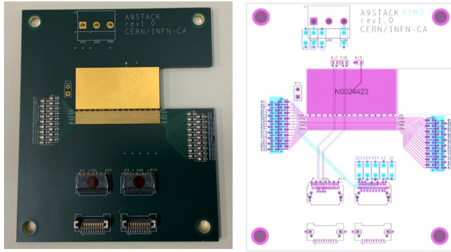
Figure 3.11: Left: the first prototype of the A9 stack carrier board. Right: carrier board layout
