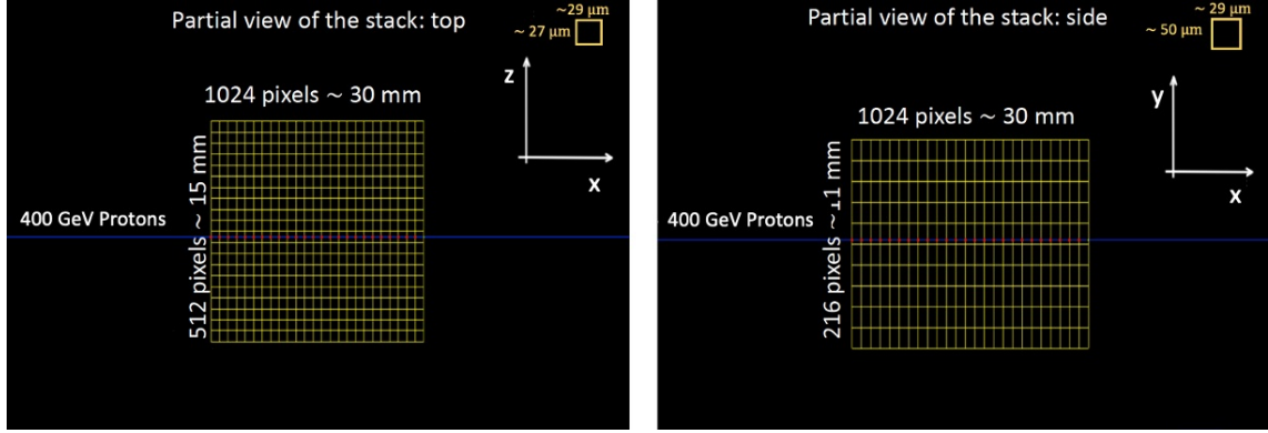
Figure 5.1: Partial view of the simulated stack on Geant4: left from above, right from side.
