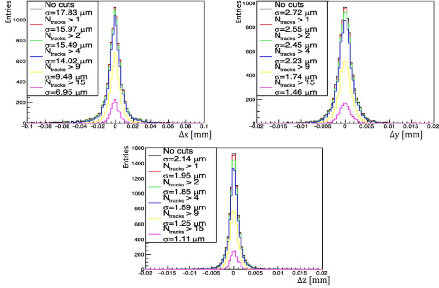
Figure 5.21: Distribution of the residuals of the reconstructed vertices with different cuts on N_{\text{tr}} .
