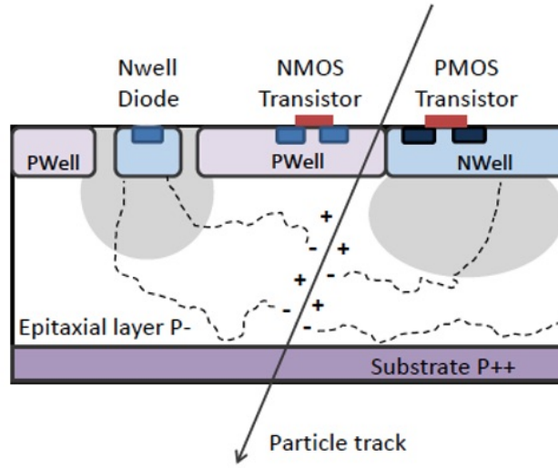
Figure 2.2: Scheme of a Monolithic Active Pixel Sensor.
