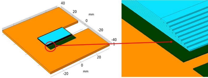
Figure 4.3: Left: Simulation model of A9 stack with the carrier board. The silicon sensor is shown in blue, the copper strip in green and the carrier board in orange. Right: Magnified view of the nine ALPIDE sensors in the A9 stack placed in a staggered manner.
