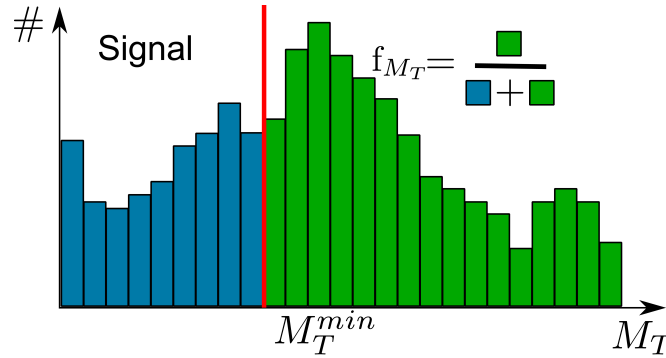
Figure 7.1: Illustration of the model-independent cross section limit determined. A series of single bins is determined by the threshold on M_T denoted as M_T^{\text{min}} .
