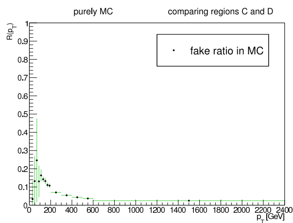
Figure 4.9: The p_T dependent fake ratio R(p_T) is produced. From the p_T \approx 200 GeV the ratio decreases from roughly 20% to \approx 5 %.
